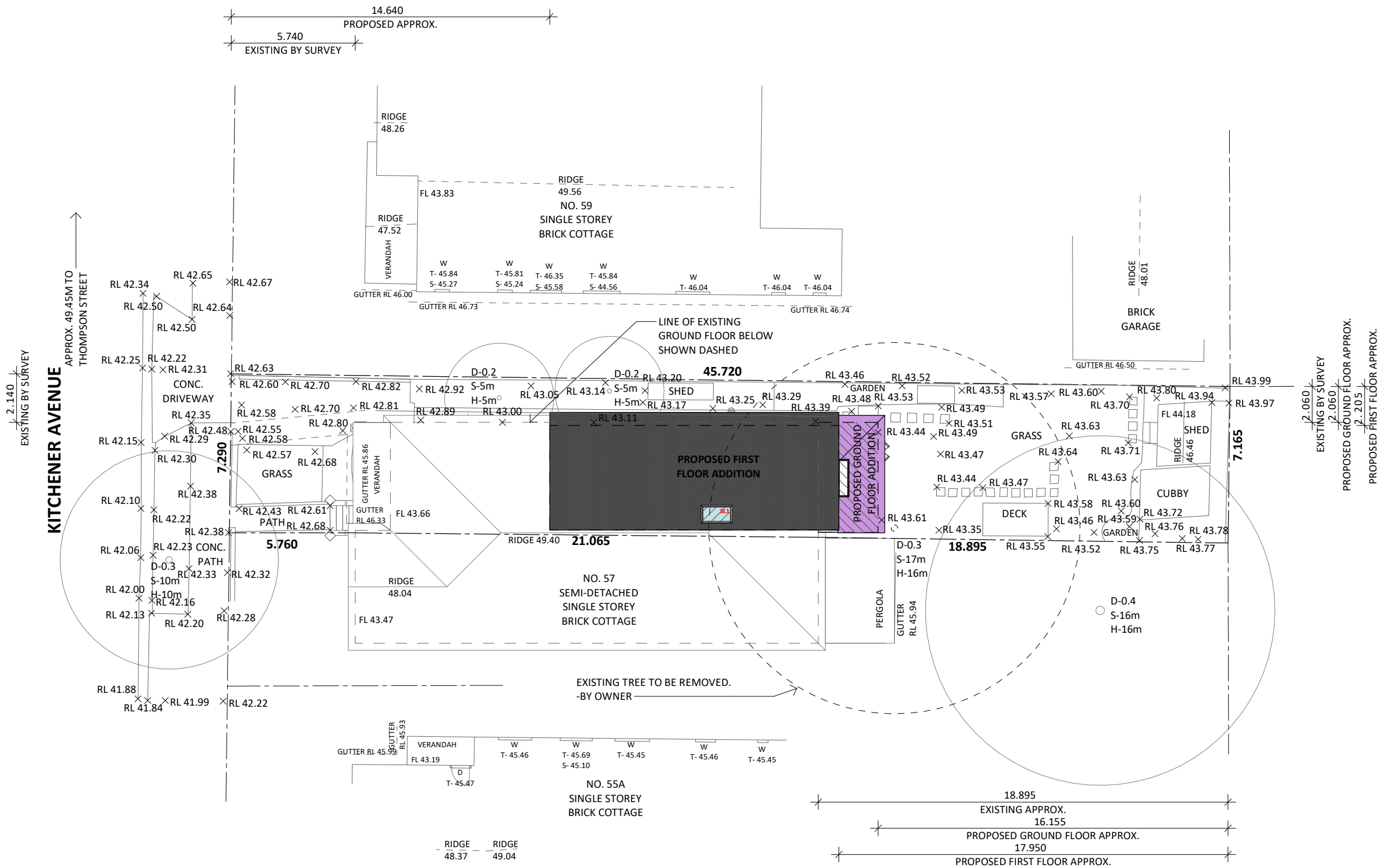
SITE PLAN
